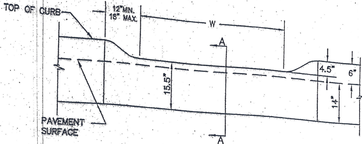
DEPRESSED CURB OPENING ELEVATION
